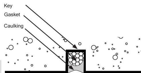
Fig. 11 Detail: control joint
