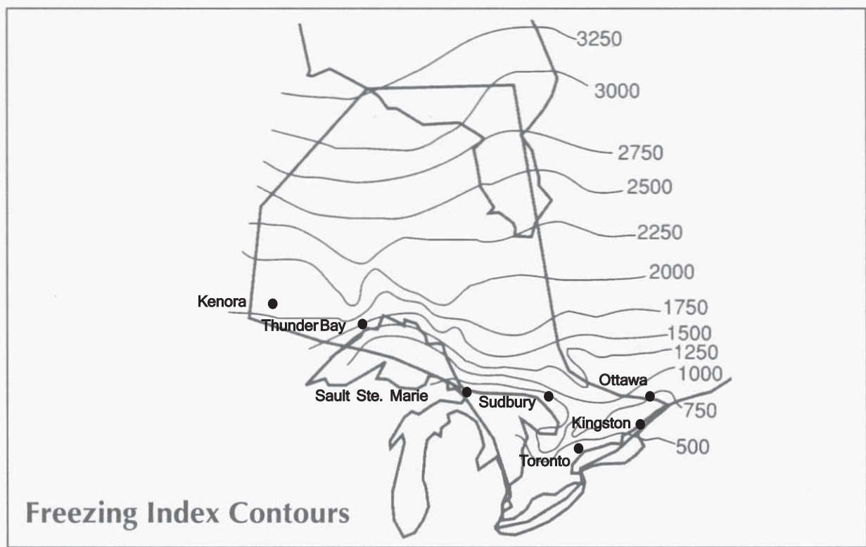
Freezing index for Ontario Fig. 3
